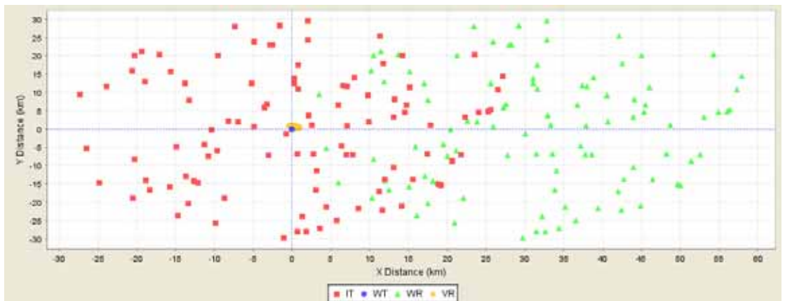
Figure 25: DTT TX into Mobile WiMAX BS RX Interference Scenario Outline from SEAMCAT
