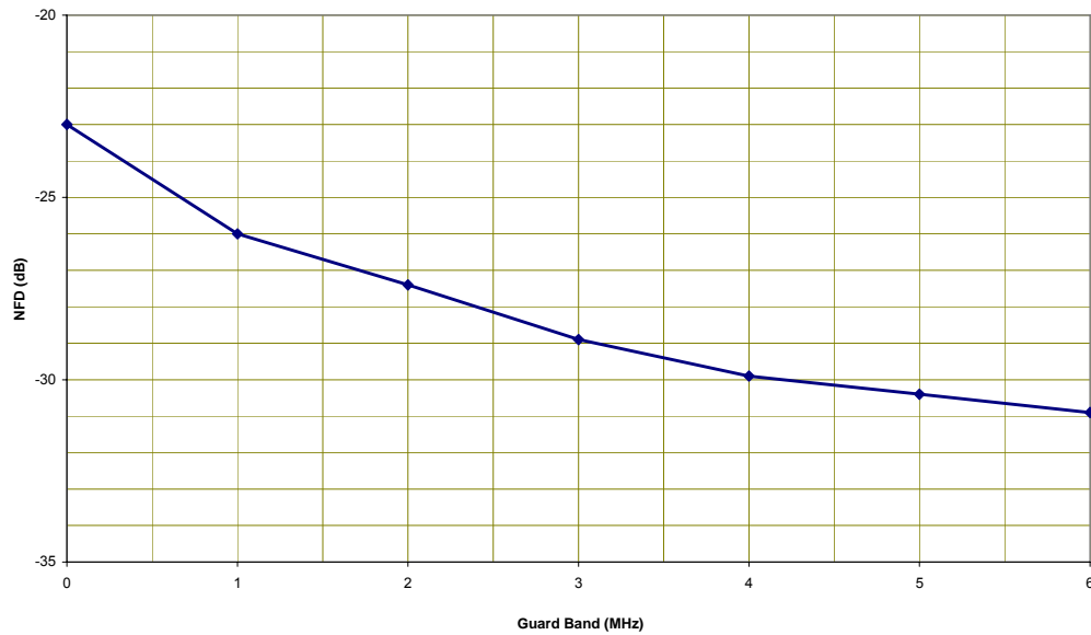
Figure 31: NFD Levels
