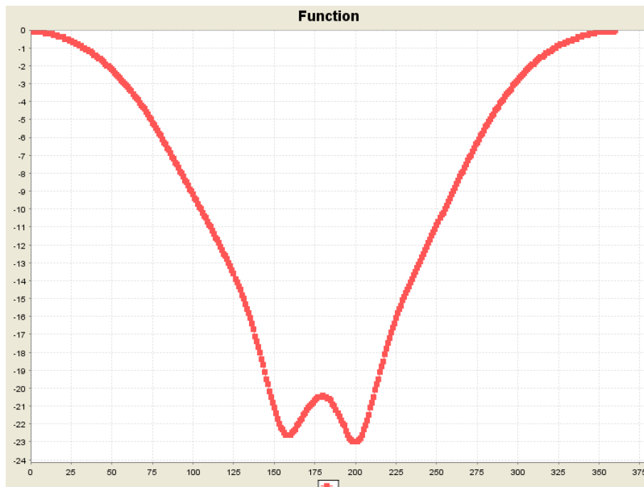
Figure 8: Mobile WiMAX BS RX Horizontal Pattern (120 Degrees Sector Antenna DB878H120E-A from www.andrew.com)
