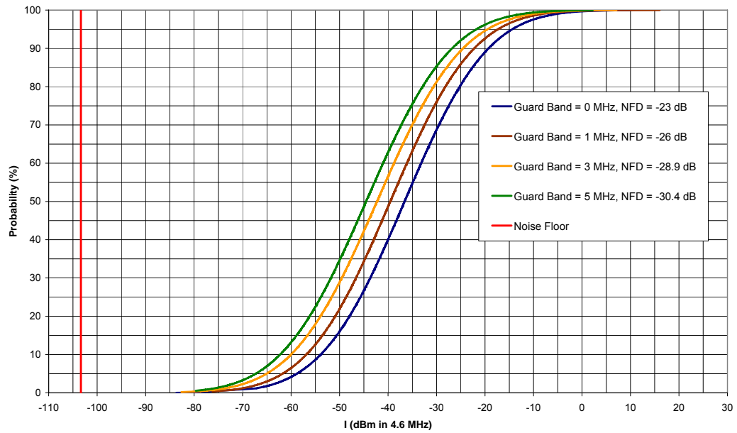
Figure 33: Interference Power CDFs
