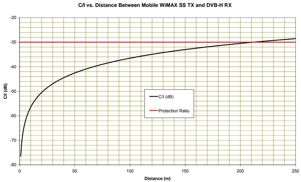
Figure 18: C/I vs. Distance Between Mobile WiMAX SS TX and DVB-H RX
