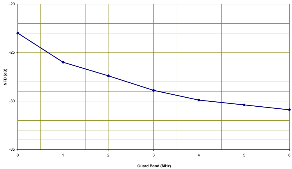
Figure 24: NFD Levels
