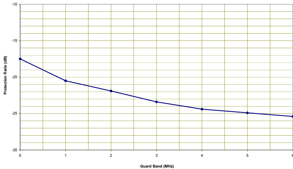
Figure 20: Protection Ratios
