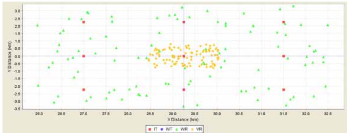
Figure 4: Mobile WiMAX BS TX into DTT RX Interference Scenario Outline from SEAMCAT (DTT RX at DTT Coverage Edge)
