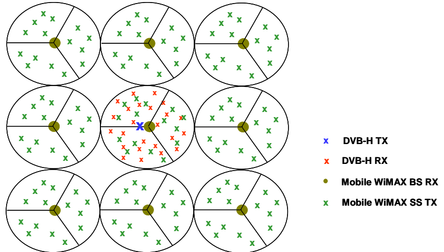
Figure 16: Interference Analysis Approach
