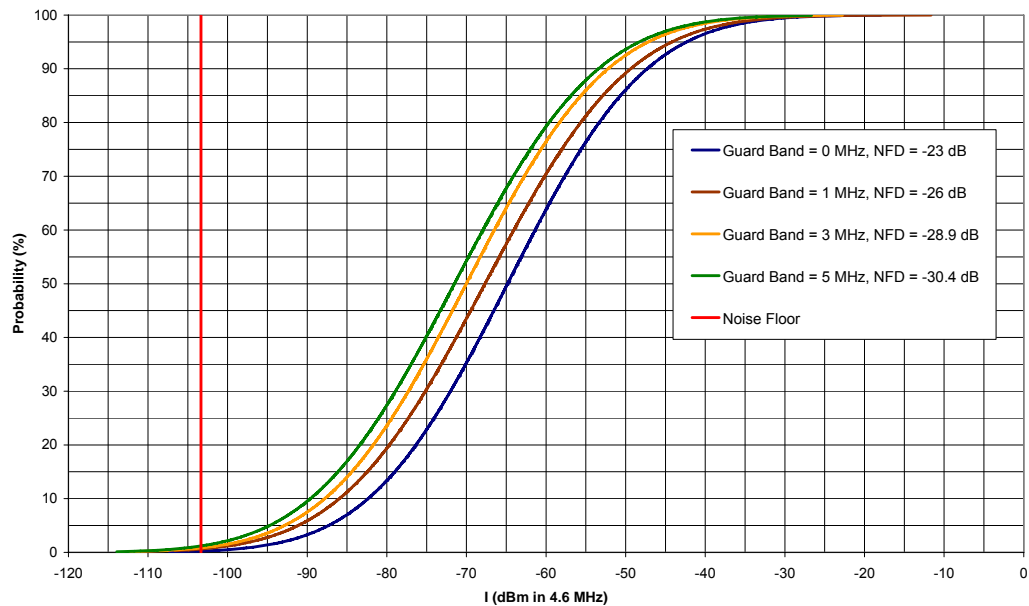
Figure 26: Interference Power CDFs
