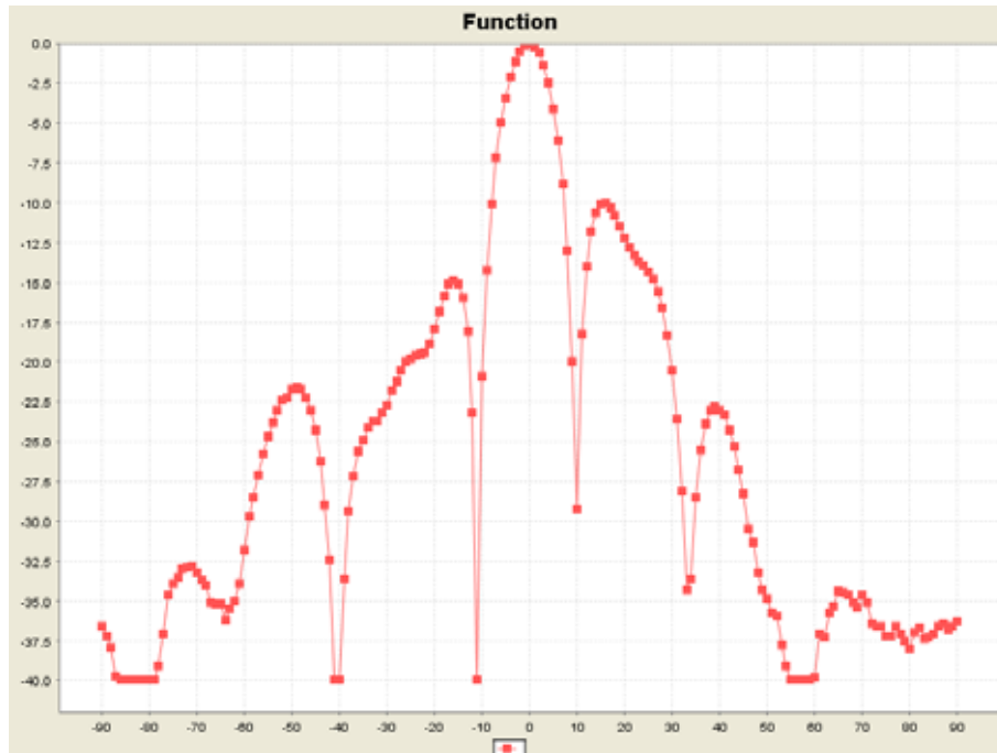
Figure 7: Mobile WiMAX BS RX Vertical Pattern (120 Degrees Sector Antenna DB878H120E-A from www.andrew.com)
