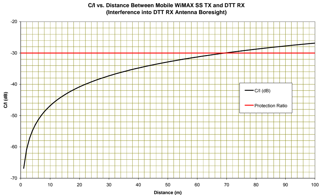
Figure 12: C/I vs. Distance Between Mobile WiMAX SS TX and DTT RX
