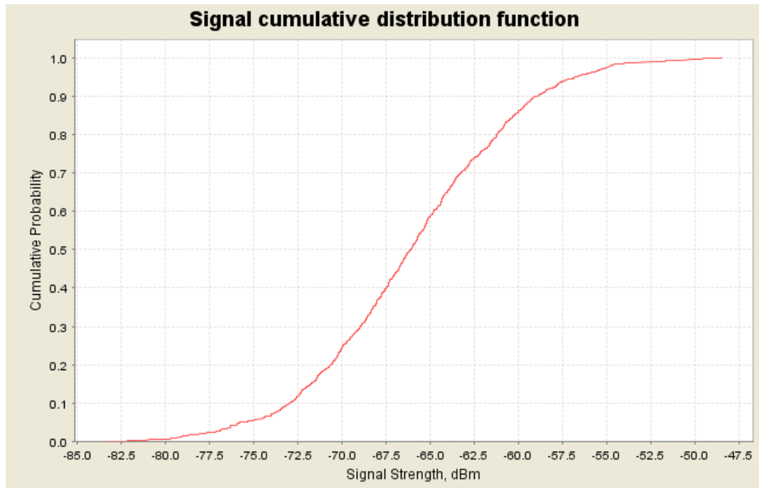
Figure 10: Wanted Power CDF at DTT RX (Mean = -66.1 dBm, Std Dev = 5.63 dB)
