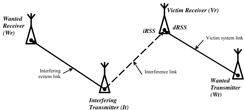
Figure 1: Main Elements of SEAMCAT Interference Scenario (Taken from SEAMCAT User Manual, http://www.ero.dk/seamcat )
