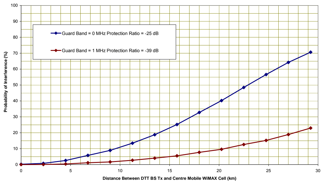
Figure 5: Interference Probabilities
