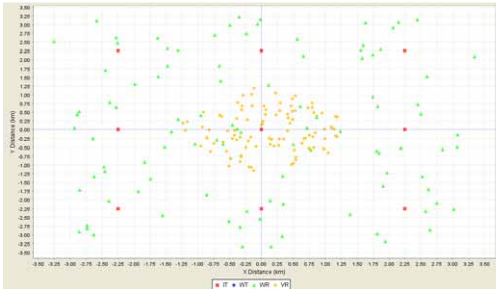
Figure 15: Mobile WiMAX BS TX into DVB-H RX Interference Scenario Outline from SEAMCAT
