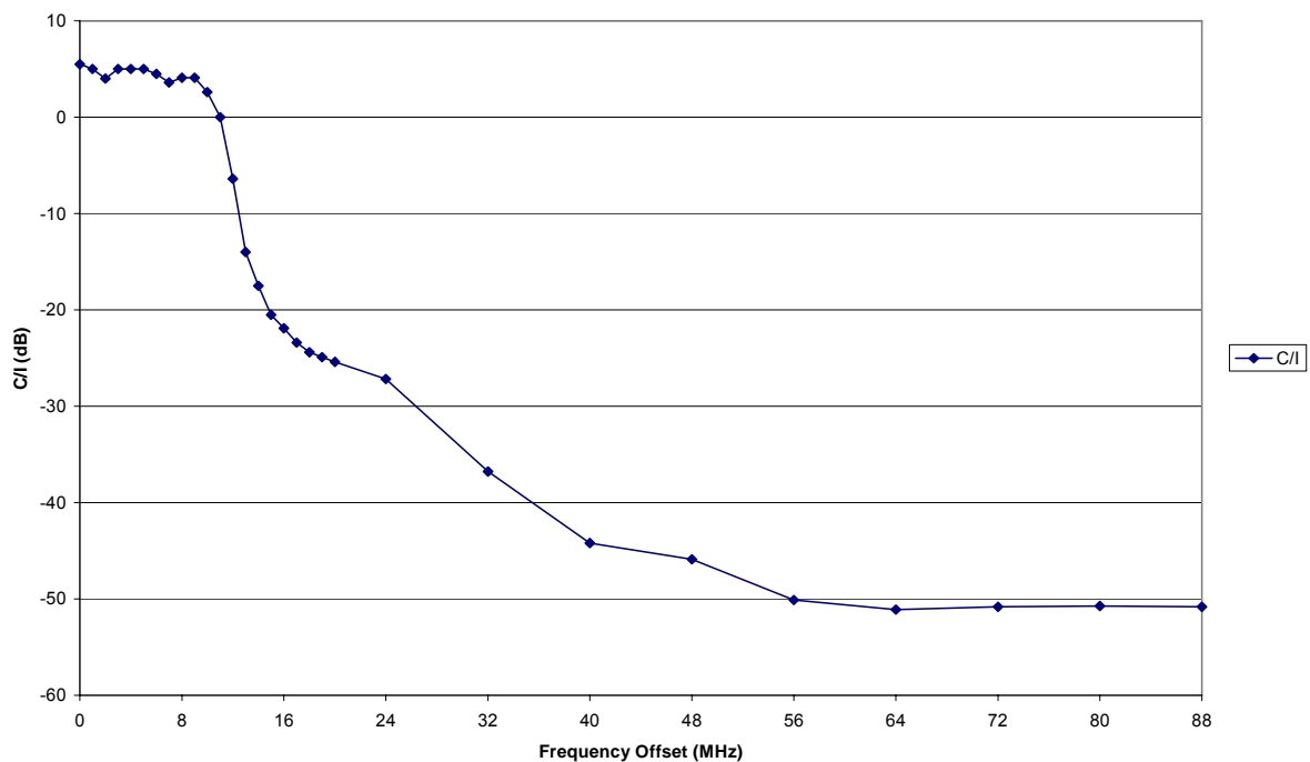
Figure 22: Extended C/I protection ratios for DTT into WiMAX
