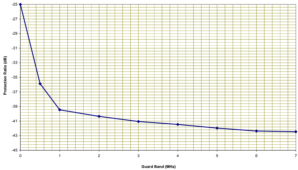
Figure 14: Protection Ratios
