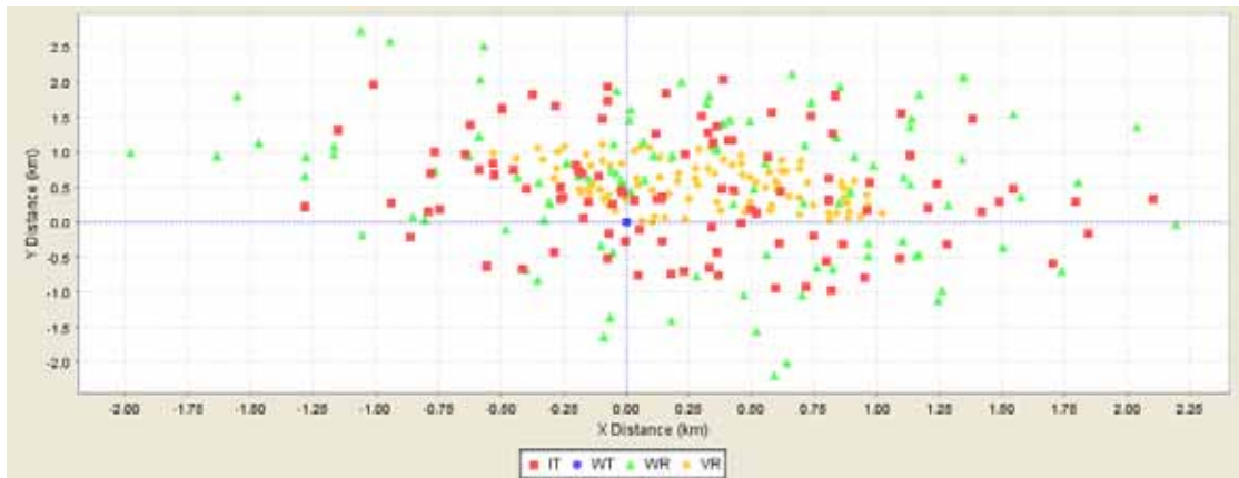
Figure 32: DVB-H TX into Mobile WiMAX BS RX Interference Scenario Outline from SEAMCAT
