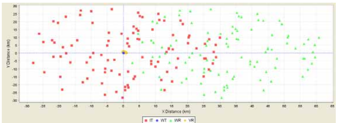
Figure 21: DTT TX into Mobile WiMAX SS RX Interference Scenario Outline from SEAMCAT
