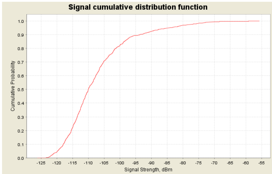
Figure 11: Interference Power CDF at DTT RX (Mean = -107.53 dBm, Std Dev = 10.58 dB)
