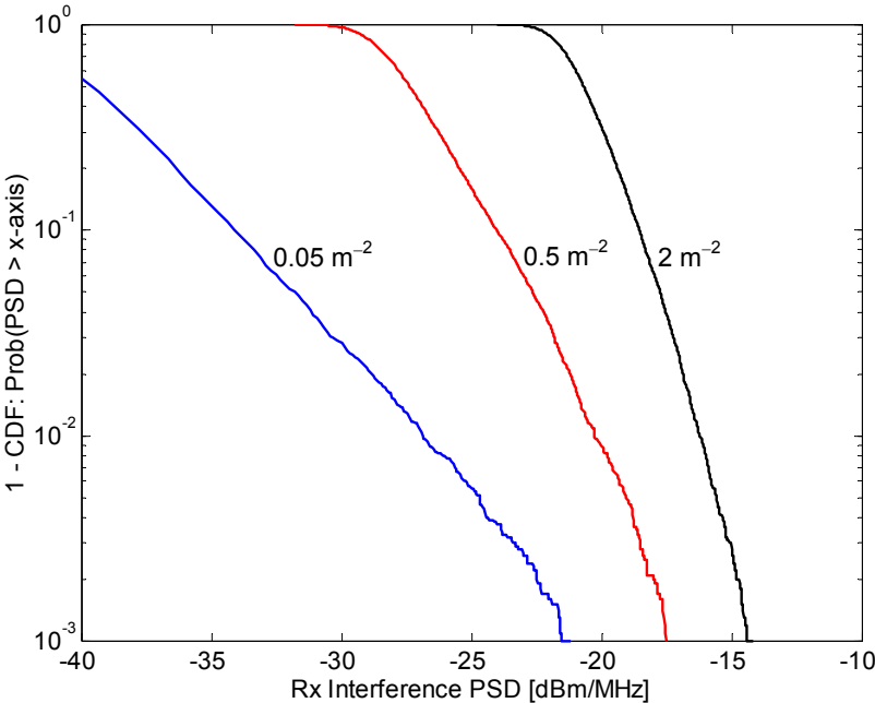
Figure A3.1. Statistics for aggregate interference PSD at 2 GHz. EIRP of 0 dBm/MHz, minimum distance of 0.15 m, activity factor of 100%.
