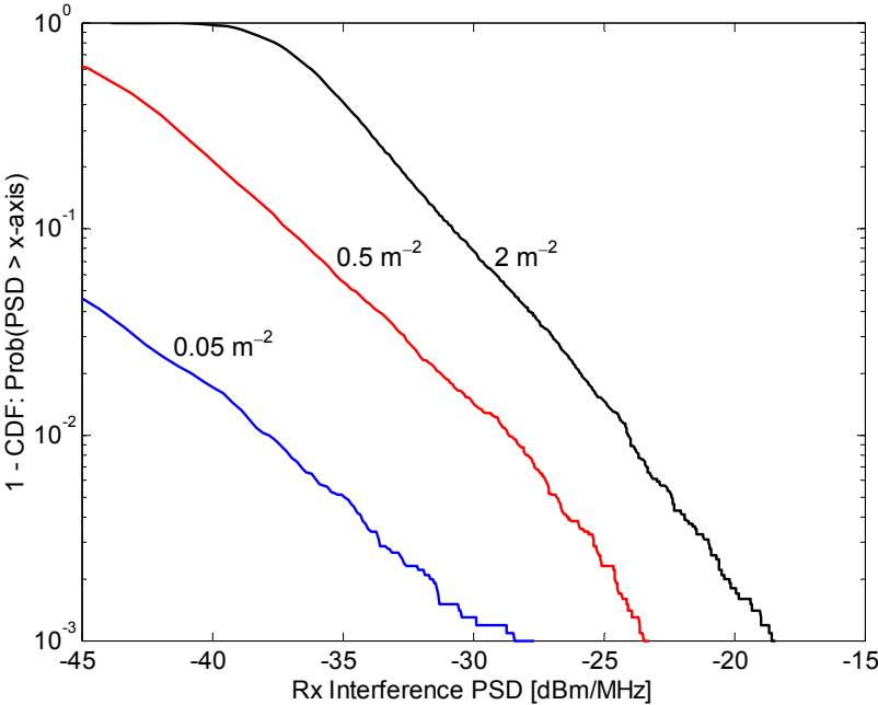
Figure A3.2. Statistics for aggregate interference PSD at 2 GHz. EIRP of 0 dBm/MHz, minimum distance of 0.15 m, activity factor of 5%.
