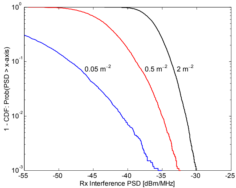
Figure A3.4. Statistics for aggregate interference PSD at 2 GHz. EIRP of 0 dBm/MHz, minimum distance of 1 m, activity factor of 5%.
