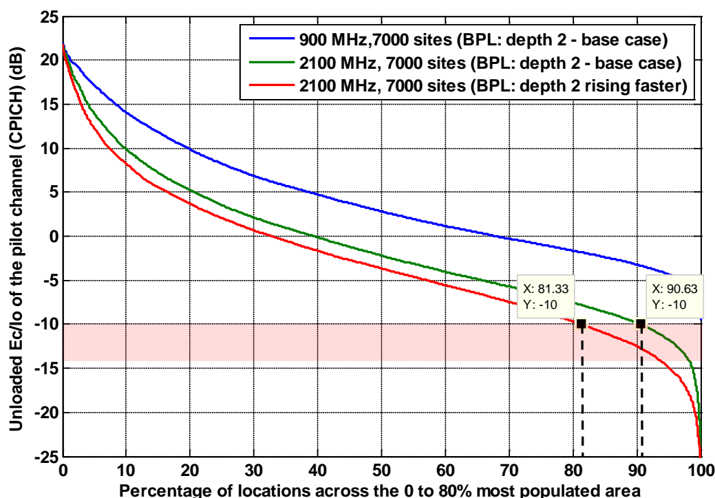
Figure A1.8: E_c/I_0 for a UMTS900 network with 7,000 sites distributed over the 80% population area compared with 7,000 sites UMTS2100 network over the same area. BPL: depth 2, base case and rising faster with frequency.
