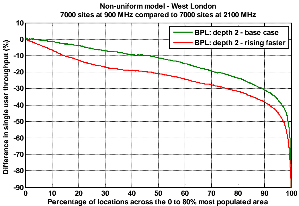
Figure A6.4: Percentage difference in throughput for a UMTS900 network with 7,000 sites distributed over the 80% population area compared with a 7,000 site UMTS2100 MHz network over the same area. BPL: depth 2, base case and rising faster with frequency.
