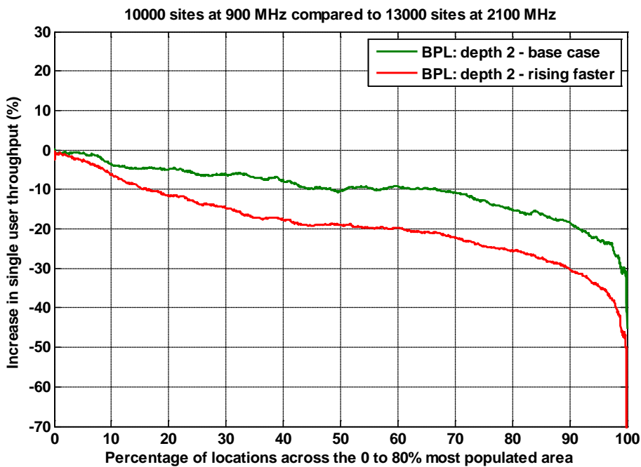
Figure A1.30: Percentage difference in throughput for a UMTS900 network with 10,000 sites distributed over the 80% population area compared with 13,000 sites at UMTS2100 over the same area. BPL: depth 2, base case and rising faster with frequency.
