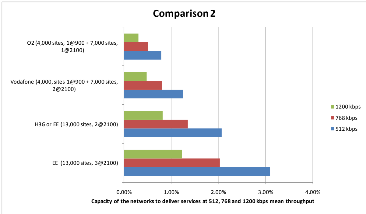
Figure A1.10: Data capacity: users supported concurrently at throughput of 0.512, 0.768 and 1.2 Mbps for Vodafone and O2 with 4,000 sites at 900 MHz and 7,000 sites at 2100 MHz and for EE and H3G with 13,000 sites at 2100 MHz distributed over the 80% population area (BPL: depth 2, base case).
