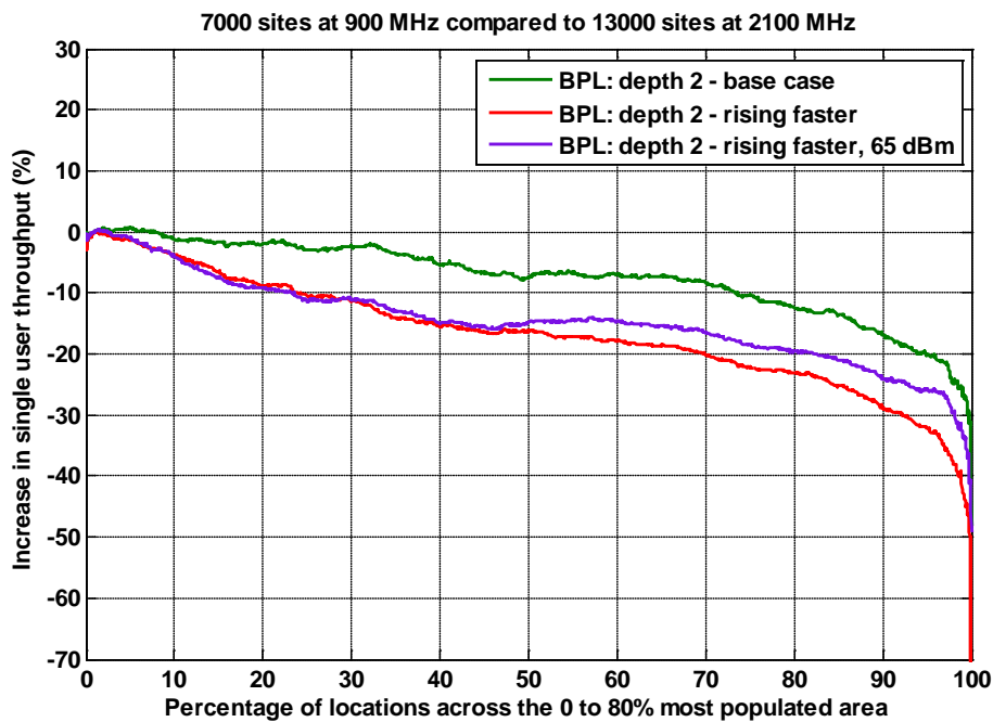
Figure A1.20: Percentage difference in throughput for a UMTS900 network with 7,000 sites distributed over the 80% population area compared with 13,000 sites at UMTS2100 over the same area. BPL: depth 2, base case and rising faster with frequency, plus 2100 MHz power increase (to 65 dBm).
