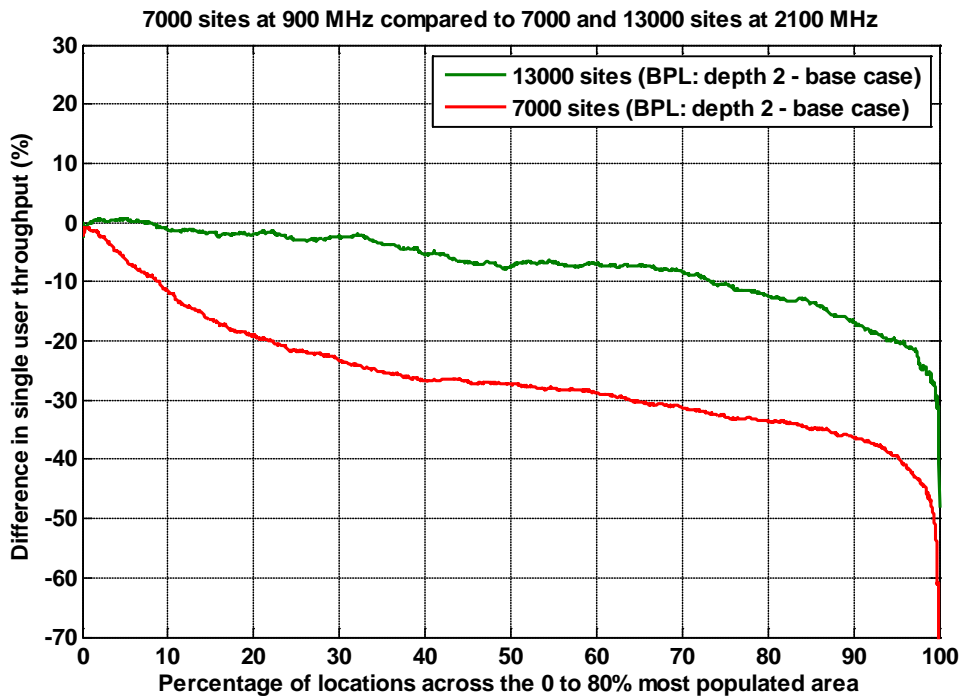
Figure A2.4: Increase in the throughput for a 900MHz compared to 2100MHz network (equal number of sites)
