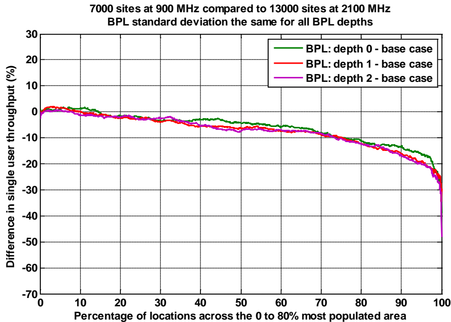
Figure A1.23: Percentage difference in throughput for UMTS900 network with 7,000 sites distributed over the 80% population area compared with 13,000 sites at UMTS2100 over the same area. BPL depths 0, 1 and 2 base case and BPL standard deviation the same for all BPL depths
