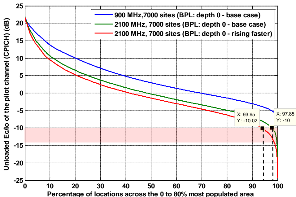
Figure A1.43: E_c/I_0 for a UMTS900 network with 7,000 sites distributed over the 80% population area compared with a 7,000 site UMTS2100 network over the same area. BPL: depth 0, base case and rising faster with frequency.
