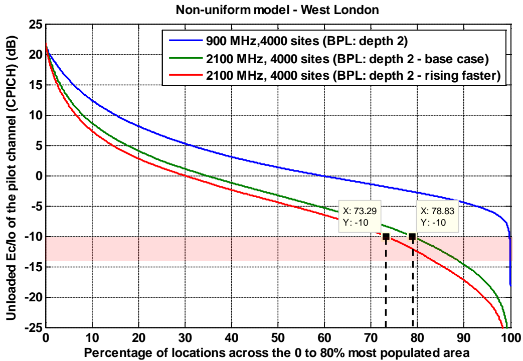
Figure A6.9: E_c/I_o for a UMTS900 network with 4,000 sites distributed over the 80% population area compared with a 4,000 site UMTS2100 network over the same area. BPL: depth 2, base case and rising faster with frequency.
