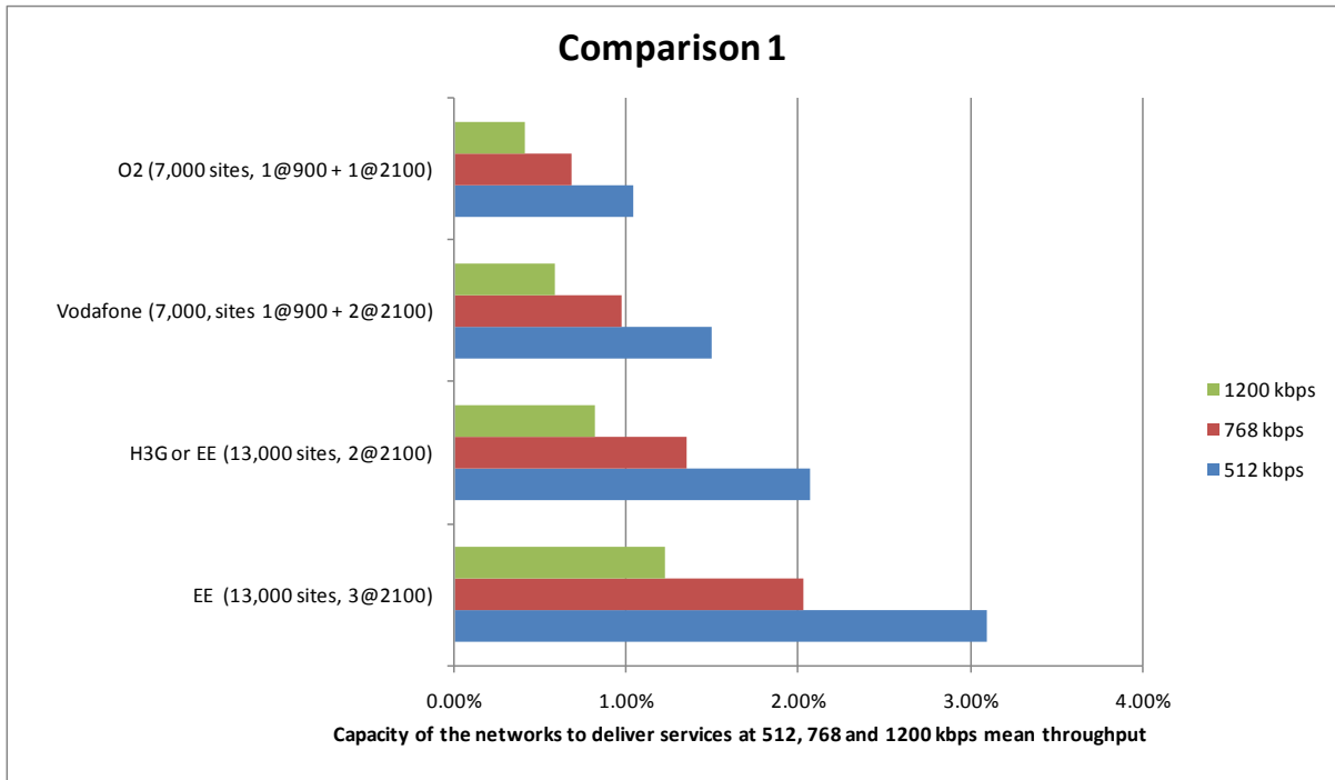
Figure A1.9: Data capacity: users supported concurrently at throughput of 0.512, 0.768 and 1.2 Mbps for Vodafone and O2 with 7,000 sites at 900 MHz and 2100 MHz and for EE and H3G with 13,000 sites at 2100 MHz distributed over the 80% population area (BPL: depth 2, base case).
