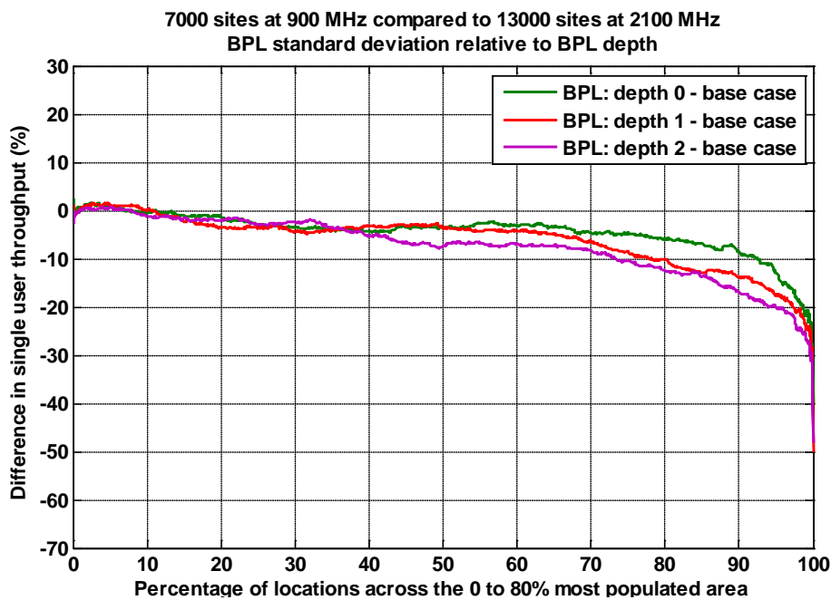
Figure A1.21: Percentage difference in throughput for UMTS900 network with 7,000 sites distributed over the 80% population area compared with 13,000 sites at UMTS2100 over the same area. BPL depths 0, 1 and 2 base case and BPL standard deviation relative to BPL depth.
