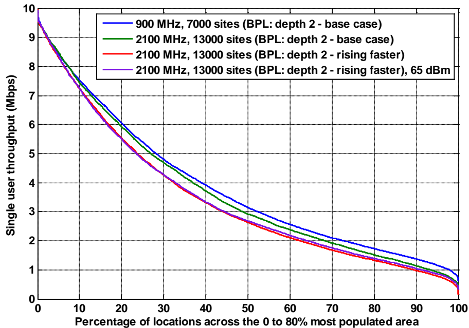
Figure A1.19: Throughput for a UMTS900 network with 7,000 sites distributed over the 80% population area compared with a 13,000 site UMTS2100 MHz network over the same area. BPL: depth 2, base case and rising faster with frequency, plus 2100 MHz power increase (to 65 dBm).
