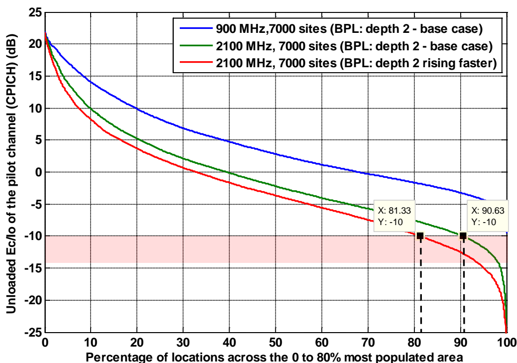
Figure A2.5: Pilot channel strength for a 900MHz network compared to a 2100MHz network (equal number of sites)
