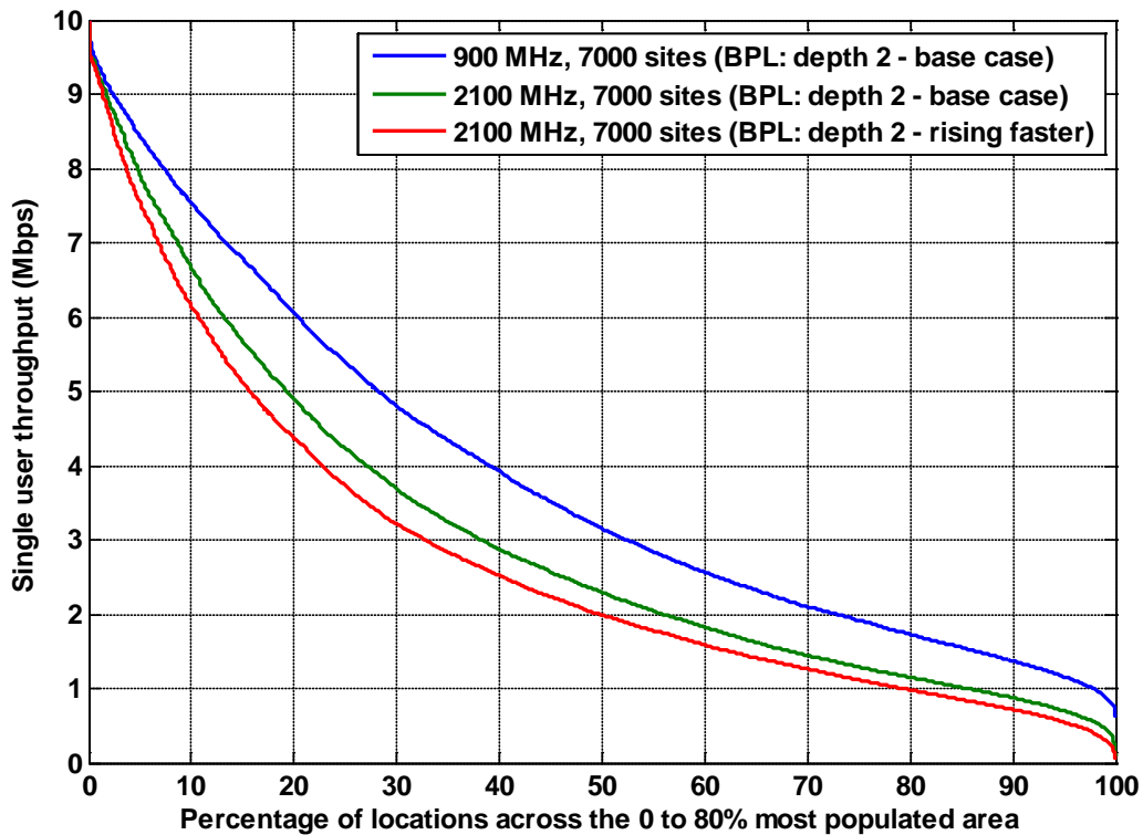
Figure A1.5: Throughput for a UMTS900 network with 7,000 sites distributed over the 80% population area compared with a 7,000 site UMTS2100 network over the same area. BPL: depth 2, base case and rising faster with frequency.
