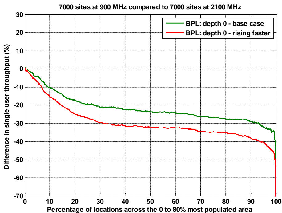
Figure A1.34: Percentage difference in throughput for a UMTS900 network with 7,000 sites distributed over the 80% population area compared with 7,000 sites at UMTS2100 over the same area. BPL: depth 0, base case and rising faster with frequency.
