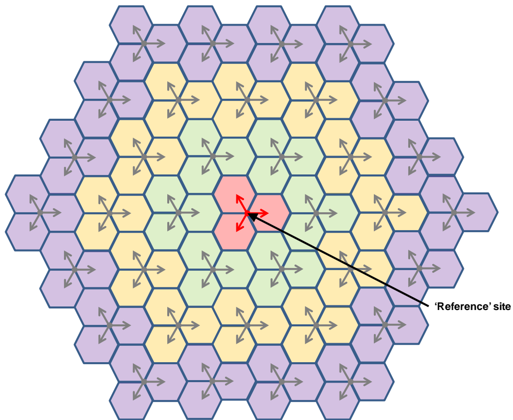
Figure A5.2: Layout of the base station array
