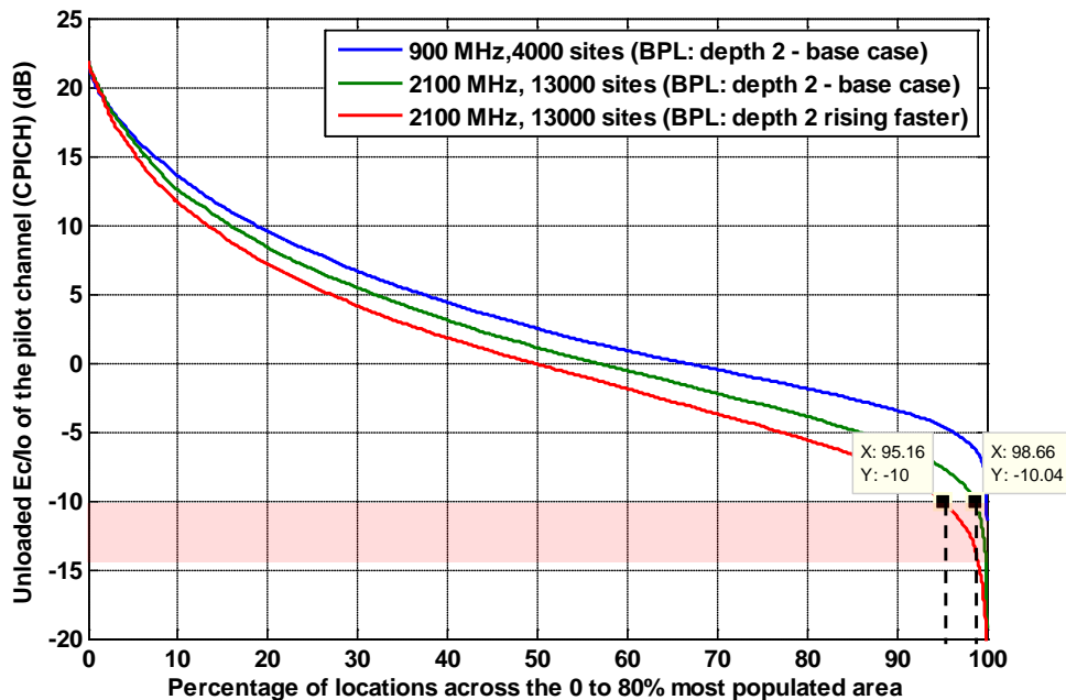
Figure A1.39: E_c/I_o for a UMTS900 network with 4,000 sites distributed over the 80% population area compared with a 13,000 site UMTS2100 network over the same area. BPL: depth 2, base case and rising faster with frequency.
