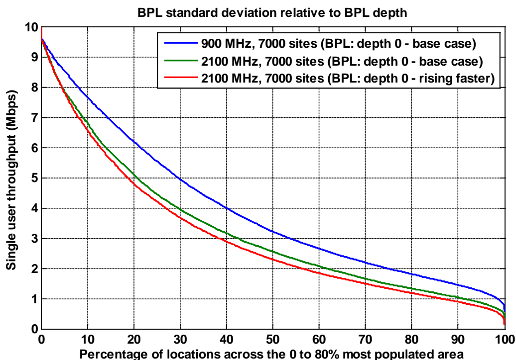
Figure A1.6: Throughput for a UMTS900 network with 7,000 sites distributed over the 80% population area compared with a 7,000 site UMTS2100 network over the same area. BPL: depth 0, base case and rising faster with frequency where the BPL standard deviation is relative to the depth.
