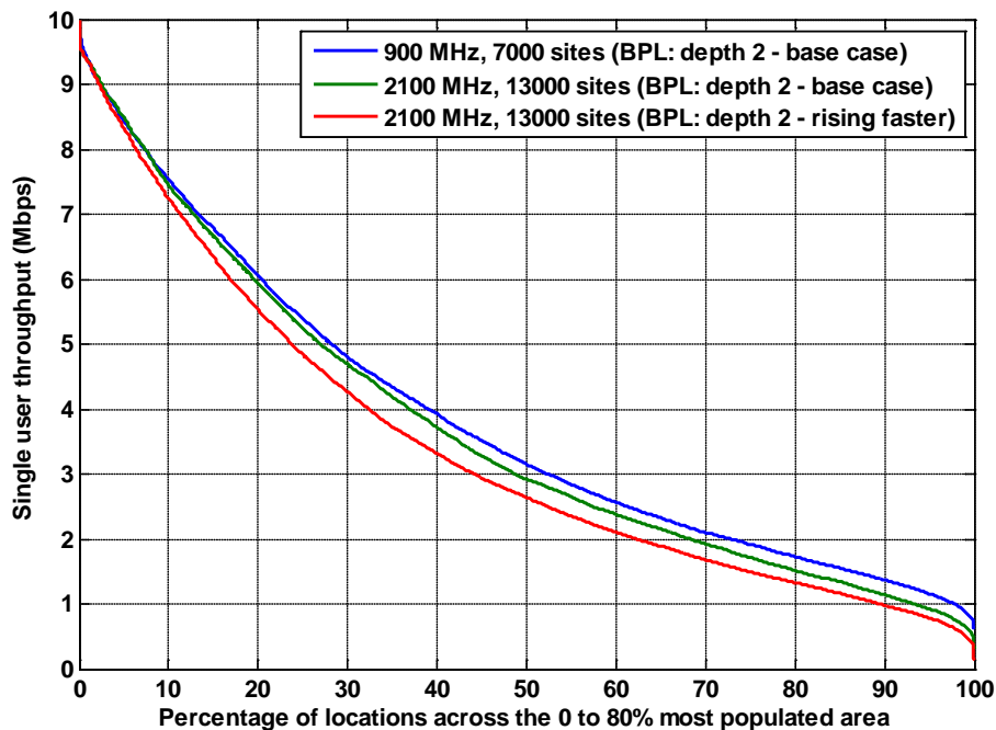
Figure A1.17: Throughput for a UMTS900 network with 7,000 sites distributed over the 80% population area compared with a 13,000 site UMTS2100 MHz network over the same area. BPL: depth 2, base case and rising faster with frequency.
