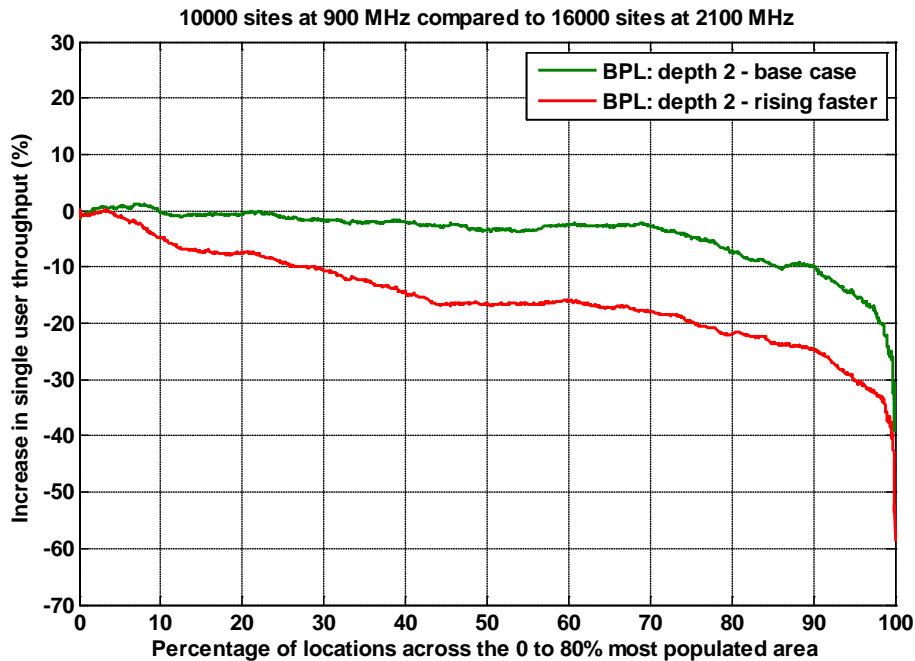
Figure A1.27: Throughput for a UMTS900 network with 10,000 sites distributed over the 80% population area compared with a 16,000 site UMTS2100 MHz network over the same area. BPL: depth 2, base case and rising faster with frequency.
