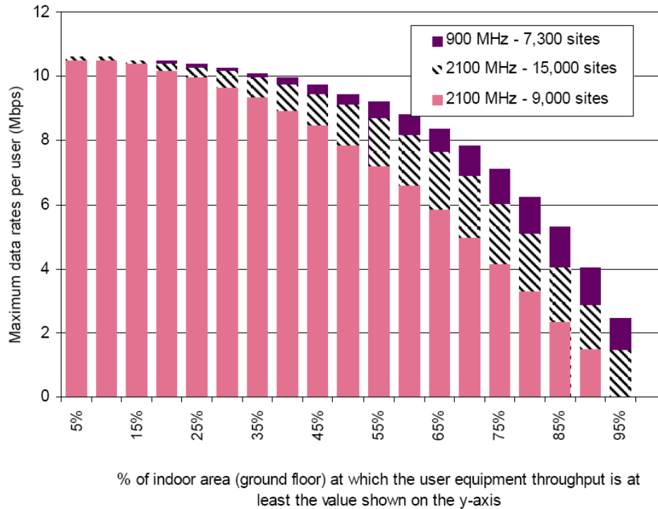
Figure A1.15: Throughput achieved by a 7,300 site UMTS900 network, a 9,000 site UMTS2100 network and a 15,000 site UMTS2100 networks – source Figure 5, February 2009 consultation.
