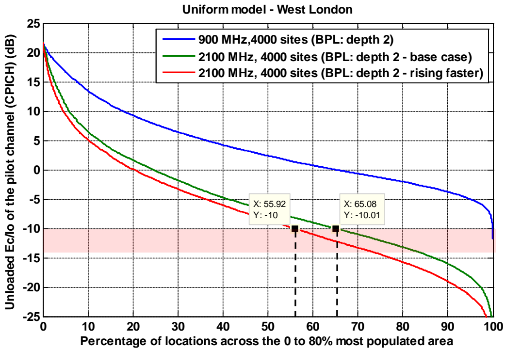
Figure A6.11: Ec/lo for a UMTS900 network with 4,000 sites distributed over the 80% population area compared with a 4,000 site UMTS2100 network over the same area. BPL: depth 2, base case and rising faster with frequency.
