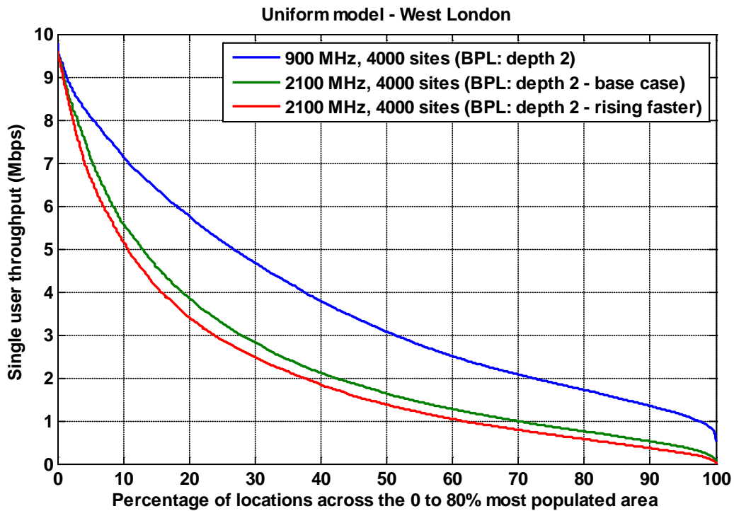
Figure A.6.5: Throughput for a UMTS900 network with 4,000 sites distributed over the 80% population area compared with a 4,000 site UMTS2100 MHz network over the same area. BPL: depth 2, base case and rising faster with frequency.
