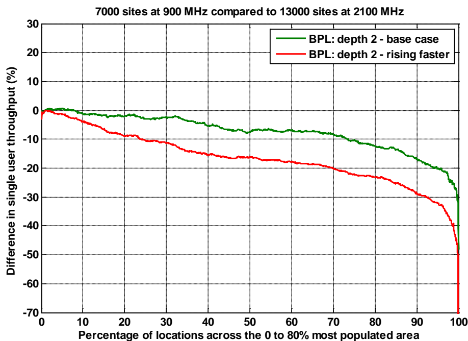
Figure A1.18: Percentage difference in throughput for a UMTS900 network with 7,000 sites distributed over the 80% population area compared with 13,000 sites at UMTS2100 over the same area. BPL: depth 2, base case and rising faster with frequency.
