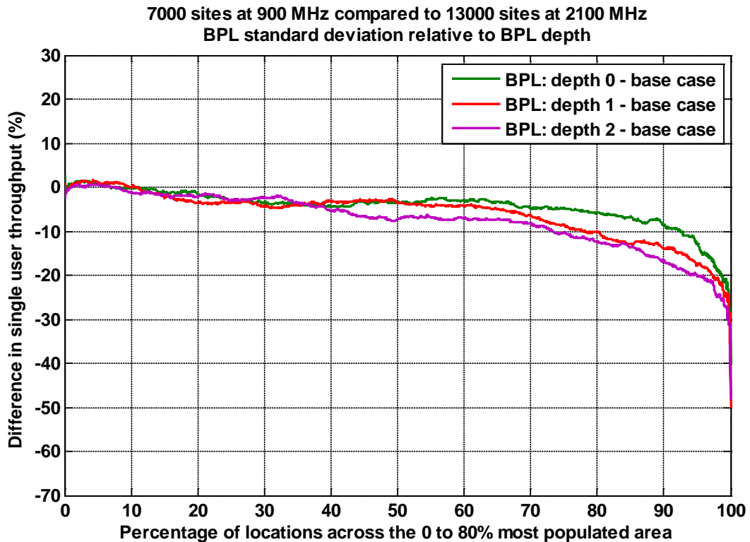
Figure A1.3: Percentage difference in throughput for UMTS900 network with 7,000 sites distributed over the 80% population area compared with 13,000 sites at UMTS2100 over the same area. BPL depths 0, 1 and 2 base case and BPL standard deviation relative to BPL depth.
