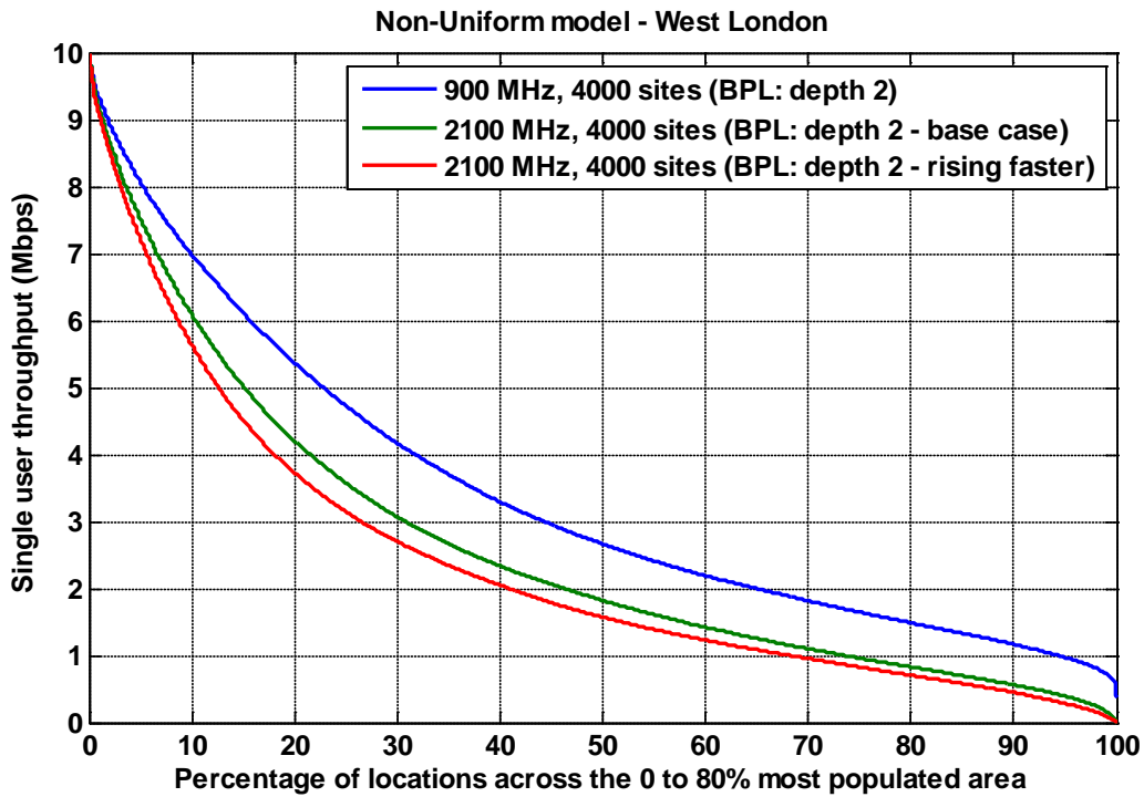
Figure A6.1: Throughput for a UMTS900 network with 4,000 sites distributed over the 80% population area compared with a 4,000 site UMTS2100 MHz network over the same area. BPL: depth 2, base case and rising faster with frequency.
