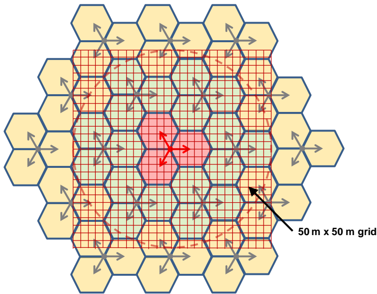
Figure A5.3: 50m x 50m grid
