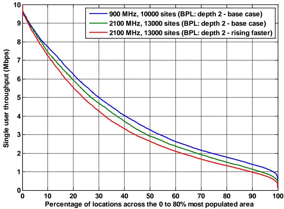
Figure A1.29: Throughput for a UMTS900 network with 10,000 sites distributed over the 80% population area compared with a 13,000 site UMTS2100 MHz network over the same area. BPL: depth 2, base case and rising faster with frequency.
