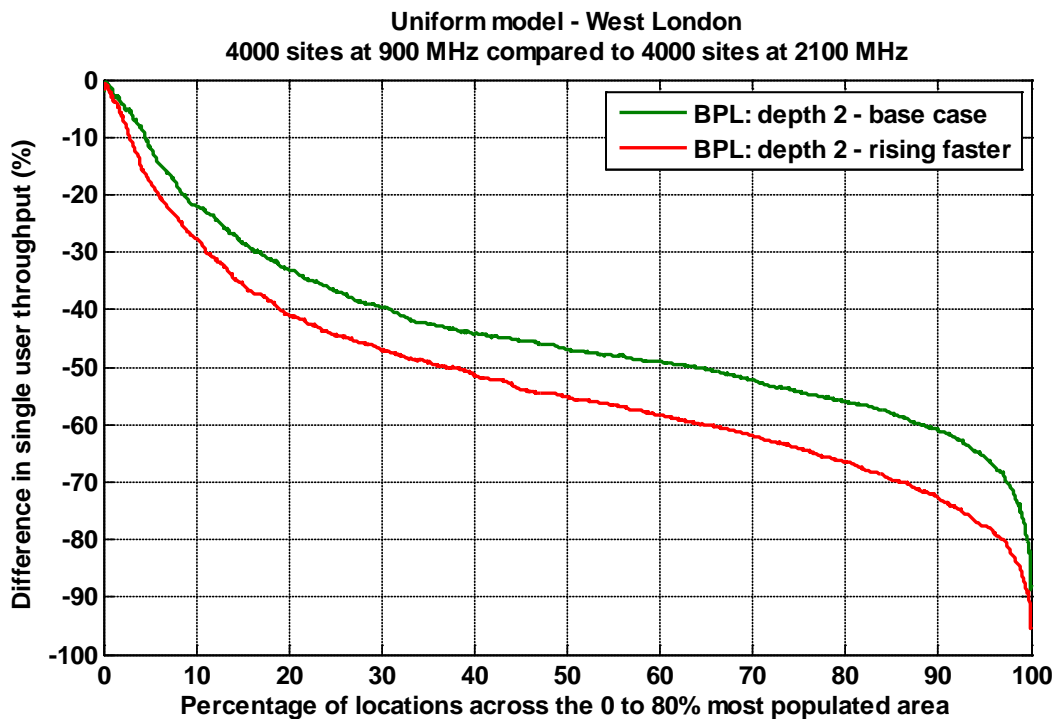
Figure A6.6: Percentage difference in throughput for a UMTS900 network with 4,000 sites distributed over the 80% population area compared with a 4,000 site UMTS2100 network over the same area. BPL: depth 2, base case and rising faster with frequency.
