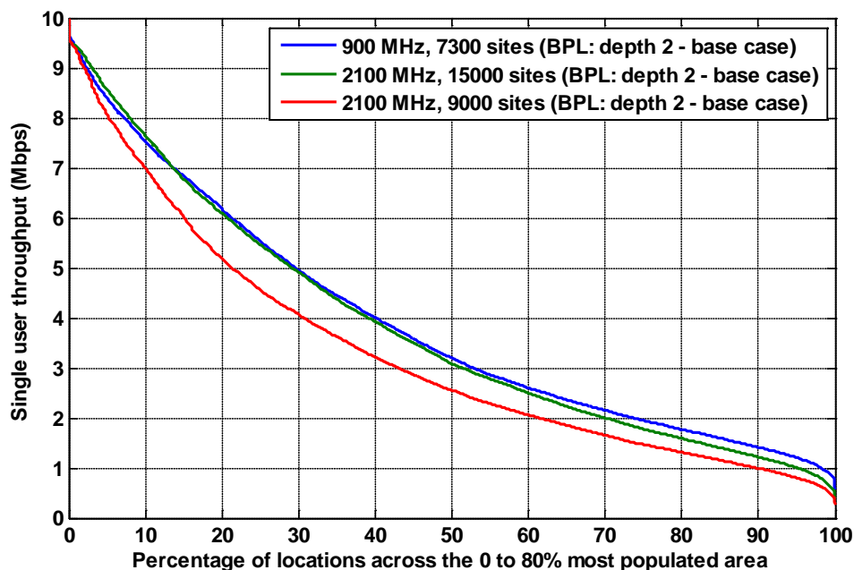
Figure A1.16: Throughput for a UMTS900 network with 7,300 sites distributed over the 80% population area compared with a 9,000 site UMTS2100 network and a 15,000 site UMTS2100 network over the same area. BPL: depth 2, base case.
