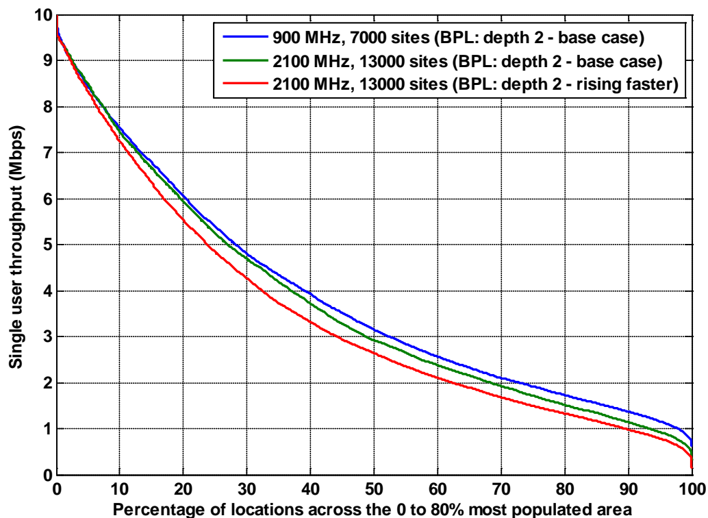
Figure A1.1: Throughput for a UMTS900 network with 7,000 sites distributed over the 80% population area compared with a 13,000 site UMTS2100 network over the same area. BPL: depth 2, base case and rising faster with frequency.
