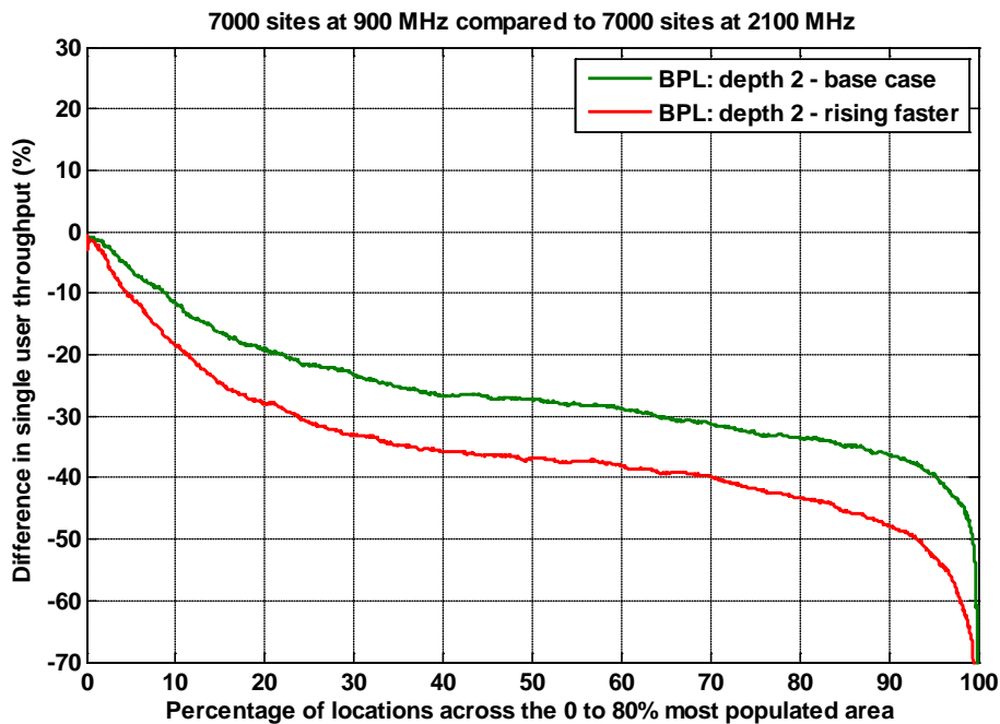
Figure A1.32: Percentage difference in throughput for a UMTS900 network with 7,000 sites distributed over the 80% population area compared with 7,000 sites at UMTS2100 over the same area. BPL: depth 2, base case and rising faster with frequency.
