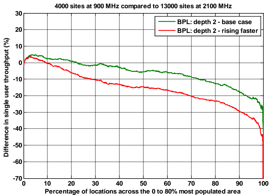
Figure A1.25: Throughput for a UMTS900 network with 4,000 sites distributed over the 80% population area compared with a 13,000 site UMTS2100 MHz network over the same area. BPL: depth 2, base case and rising faster with frequency.
