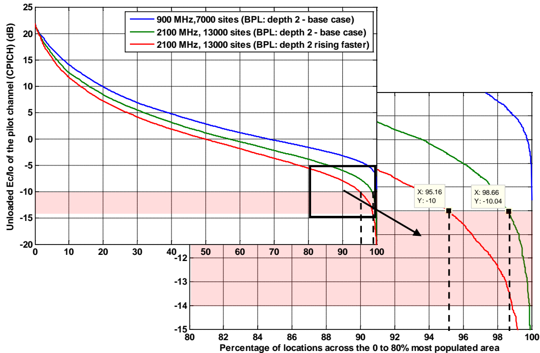
Figure A1.7: Ec/Io for a UMTS900 network with 7,000 sites distributed over the 80% population area compared with a 13,000 site UMTS2100 network over the same area. BPL: depth 2, base case and rising faster with frequency.
