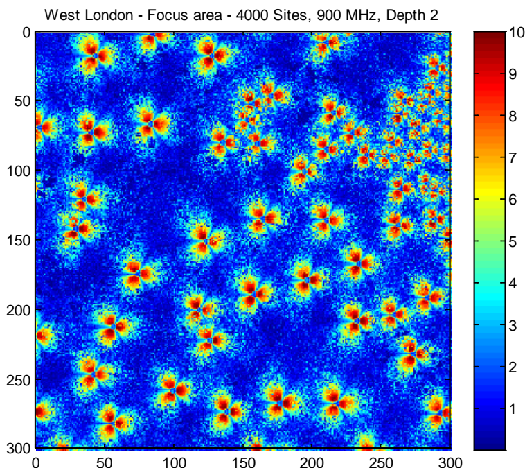
Figure A5.8: West London - Focus box – Single User Throughput (Mbps)
