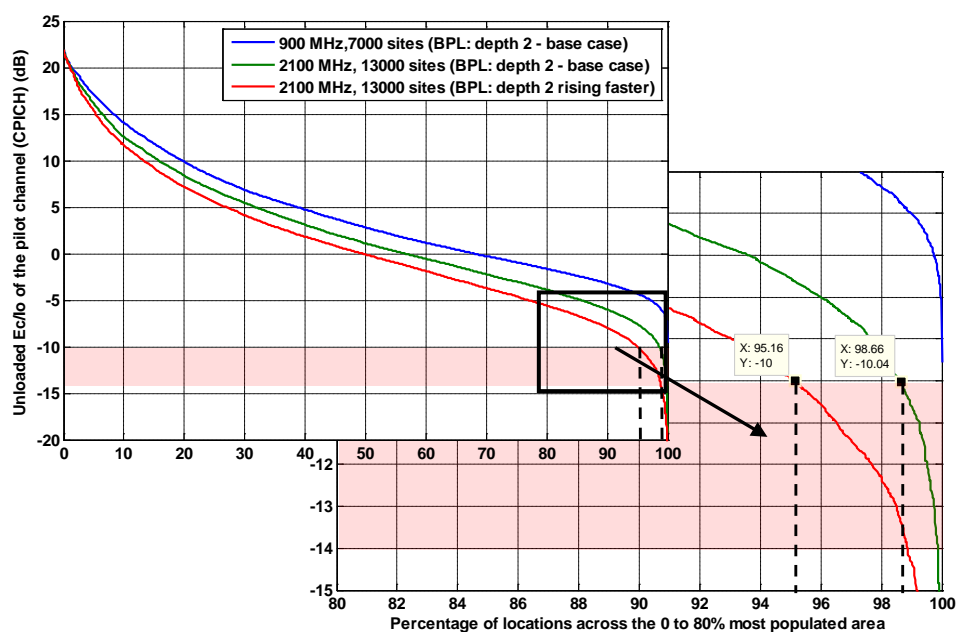
Figure A1.37: E_c/I_0 for a UMTS900 network with 7,000 sites distributed over the 80% population area compared with a 13,000 site UMTS2100 network over the same area. BPL: depth 2, base case and rising faster with frequency.
