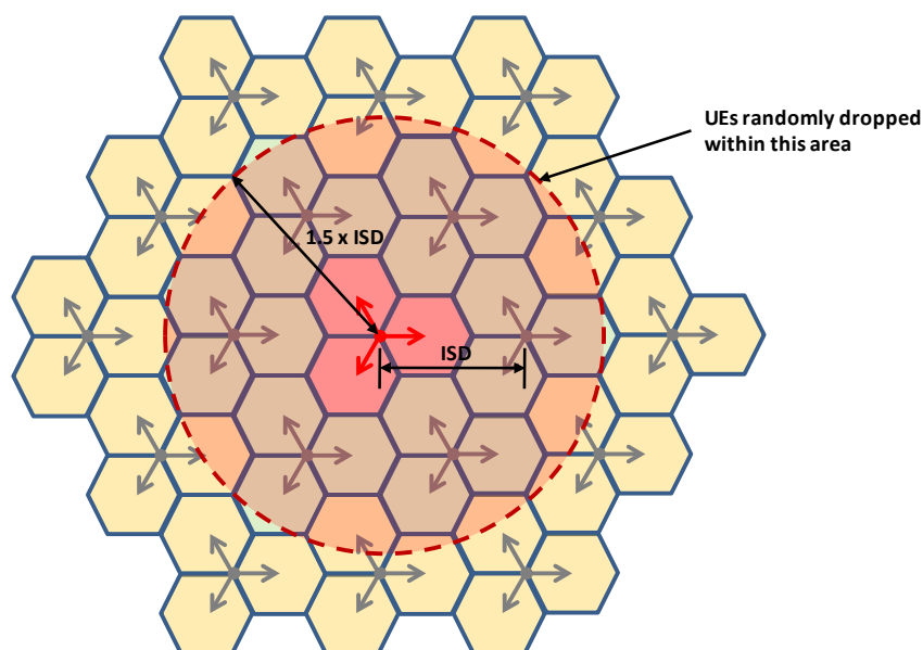
Figure A5.4: Area UEs are dropped
