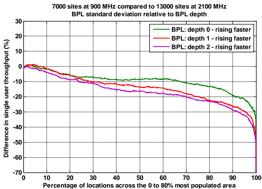
Figure A1.22: Percentage difference in throughput for UMTS900 network with 7,000 sites distributed over the 80% population area compared with 13,000 sites at UMTS2100 over the same area. BPL depths 0, 1 and 2 rising faster with frequency and BPL standard deviation relative to BPL depth.
