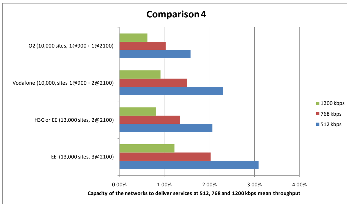
Figure A1.12: Data capacity: users supported concurrently at throughput of 0.512, 0.768 and 1.2 Mbps for Vodafone and O2 with 10,000 sites at 900 MHz and 2100 MHz and for EE and H3G with 13,000 sites at 2100 MHz distributed over the 80% population area (BPL: depth 2, base case).
