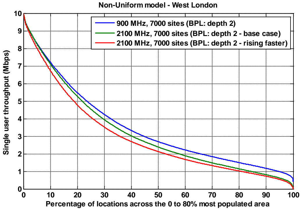
Figure A6.3: Throughput for a UMTS900 network with 7,000 sites distributed over the 80% population area compared with a 7,000 site UMTS2100 MHz network over the same area. BPL: depth 2, base case and rising faster with frequency.
