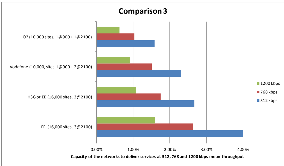
Figure A1.11: Data capacity: users supported concurrently at throughput of 0.512, 0.768 and 1.2 Mbps for Vodafone and O2 with 10,000 sites at 900 MHz and 2100 MHz and for EE and H3G with 16,000 sites at 2100 MHz distributed over the 80% population area (BPL: depth 2, base case).
