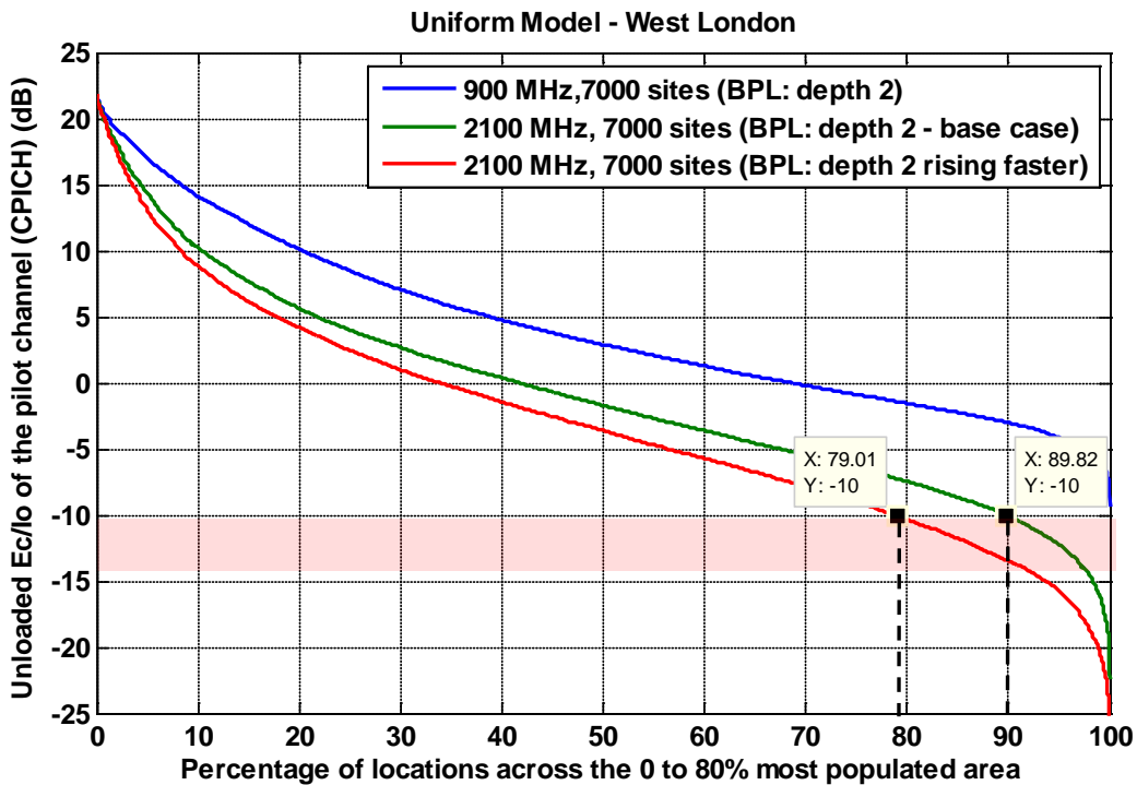
Figure A6.12: Ec/lo for a UMTS900 network with 7,000 sites distributed over the 80% population area compared with a 7,000 site UMTS2100 network over the same area. BPL: depth 2, base case and rising faster with frequency.
