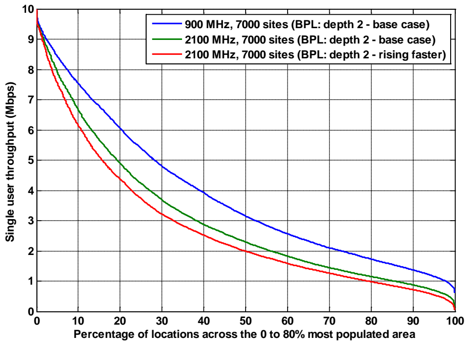
Figure A1.31: Throughput for a UMTS900 network with 7,000 sites distributed over the 80% population area compared with a 7,000 site UMTS2100 MHz network over the same area. BPL: depth 2, base case and rising faster with frequency.
