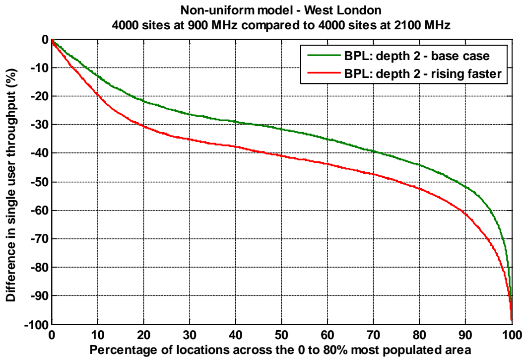
Figure A6.2: Percentage difference in throughput for a UMTS900 network with 4,000 sites distributed over the 80% population area compared with a 4,000 site UMTS2100 MHz network over the same area. BPL: depth 2, base case and rising faster with frequency.
