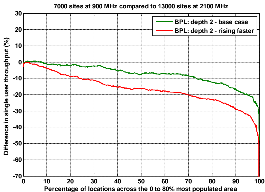
Figure A1.2: Percentage difference in throughput for a UMTS900 network with 7,000 sites distributed over the 80% population area compared with 13,000 sites at UMTS2100 over the same area. BPL: depth 2, base case and rising faster with frequency.
