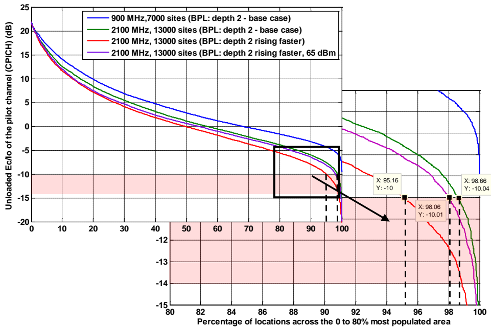
Figure A1.38: E_c/I_o for a UMTS900 network with 7,000 sites distributed over the 80% population area compared with a 13,000 site UMTS2100 network over the same area. BPL: depth 2, base case and rising faster with frequency, plus 2100 MHz power increase (65 dBm).
