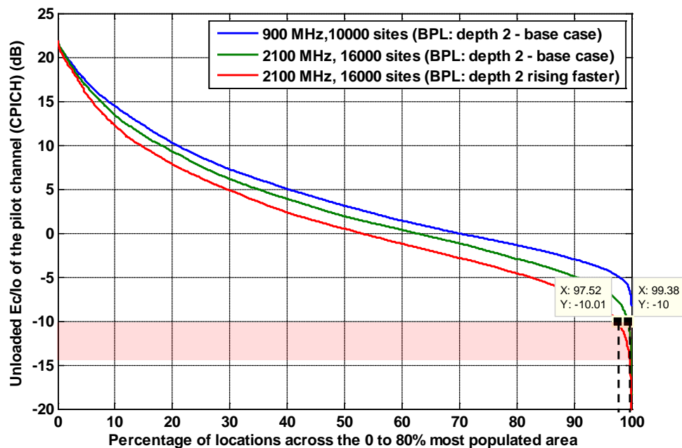
Figure A1.41: E_c/I_o for a UMTS900 network with 10,000 sites distributed over the 80% population area compared with a 16,000 site UMTS2100 network over the same area. BPL: depth 2, base case and rising faster with frequency.
