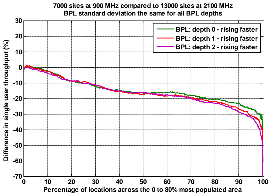
Figure A1.24: Percentage difference in throughput for UMTS900 network with 7,000 sites distributed over the 80% population area compared with 13,000 sites at UMTS2100 over the same area. BPL depths 0, 1 and 2 rising faster with frequency and BPL standard deviation the same for all BPL depths.
