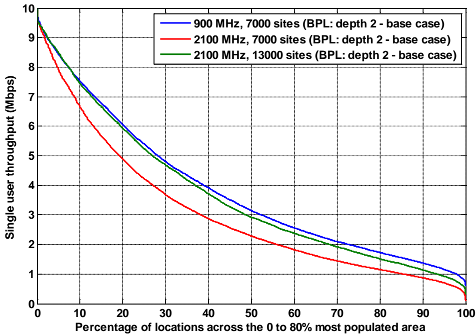
Figure A2.3: Throughput for a single user
