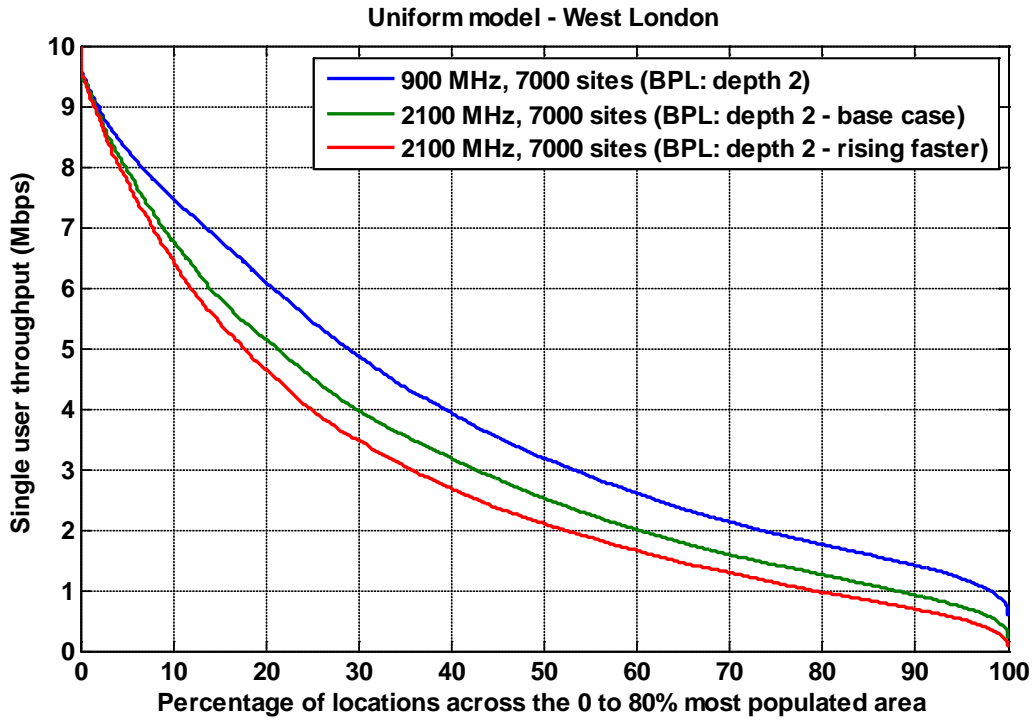
Figure A.6.7: Throughput for a UMTS900 network with 7,000 sites distributed over the 80% population area compared with a 7,000 site UMTS2100 MHz network over the same area. BPL: depth 2, base case and rising faster with frequency.
