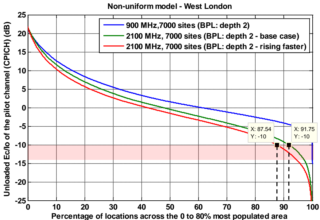
Figure A6.10: E_c/I_o for a UMTS900 network with 7,000 sites distributed over the 80% population area compared with a 7,000 site UMTS2100 network over the same area. BPL: depth 2, base case and rising faster with frequency.
