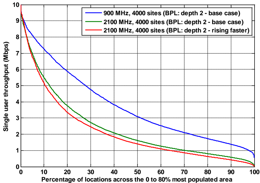
Figure A1.35: Throughput for a UMTS900 network with 4,000 sites distributed over the 80% population area compared with a 4,000 site UMTS2100 MHz network over the same area. BPL: depth 2, base case and rising faster with frequency.
