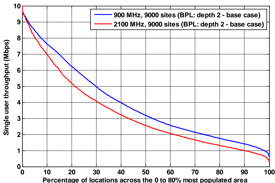
Figure A1.14: Throughput for a UMTS900 network with 9,000 sites distributed over the 80% population area compared with a 9,000 site UMTS2100 network over the same area. BPL: depth 2, base case.
