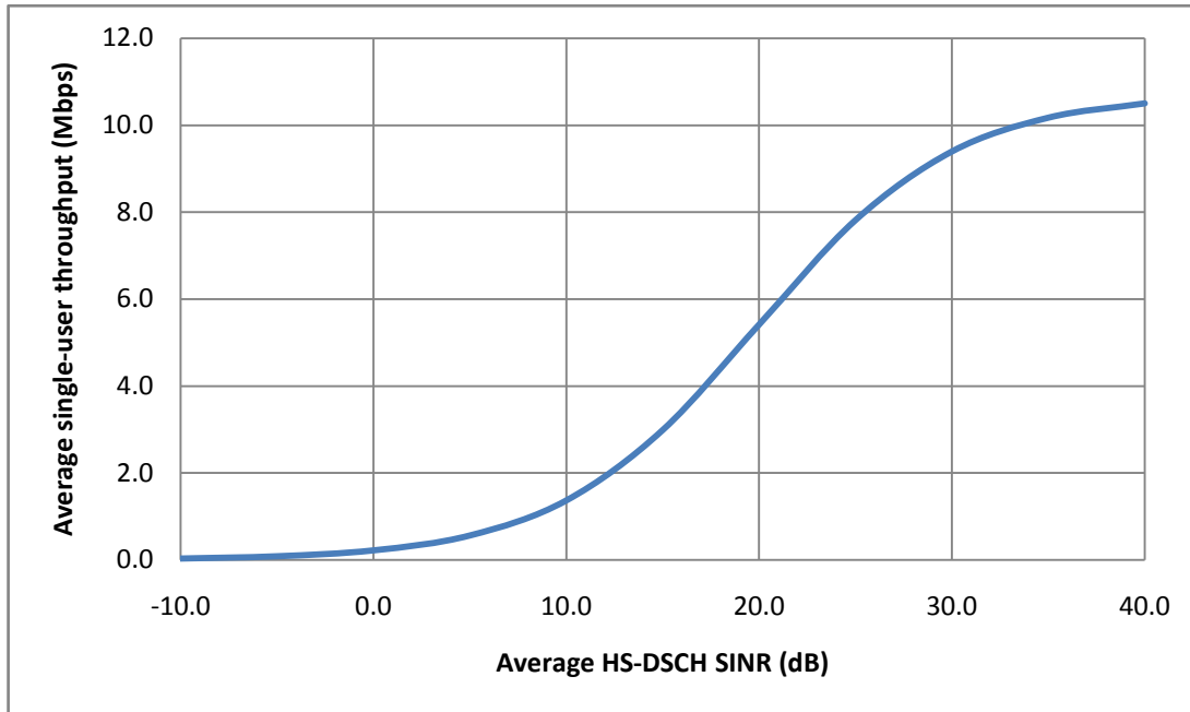
Figure A.5.6: Single user throughput mapping (15 codes)
