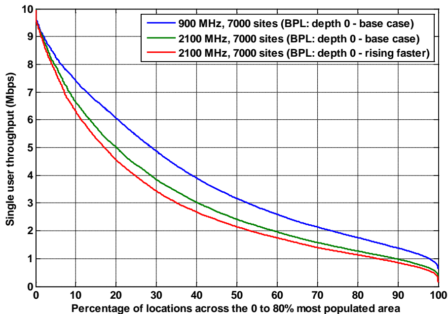
Figure A1.33: Throughput for a UMTS900 network with 7,000 sites distributed over the 80% population area compared with a 7,000 site UMTS2100 MHz network over the same area. BPL: depth 0, base case and rising faster with frequency.
