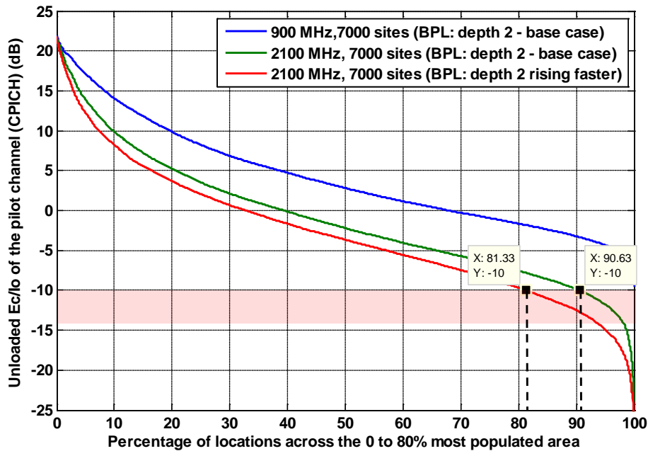
Figure A1.42: E_c/I_0 for a UMTS900 network with 7,000 sites distributed over the 80% population area compared with a 7,000 site UMTS2100 network over the same area. BPL: depth 2, base case and rising faster with frequency.
